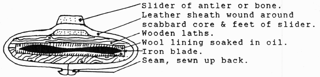
Section through a scabbard of the "slider" type.
